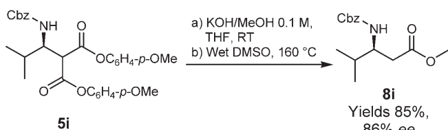
Scheme 1. Determination of absolute configuration by transesterification/decarboxylation sequence.
